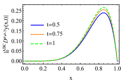
(c) The absolute ABC fractional derivative for Example 3 at \alpha = 1.9 .
