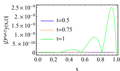
(a) The absolute ABC fractional derivative for Example 1 at \alpha = 1.9 .
