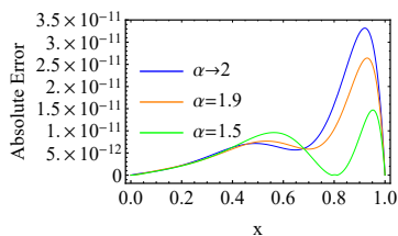
(c) The absolute error between the analytic solution and approximate solution for n = m = 10 with t = 1 .
