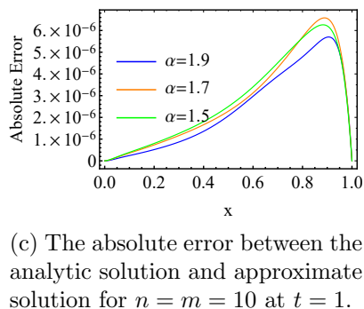
Figure 8: Graph of the absolute error between analytic solution and approximate solution of Example 3 for n = m = 10 with different values of \alpha , \mu = \gamma = 1 and fixed value of t in each case.
