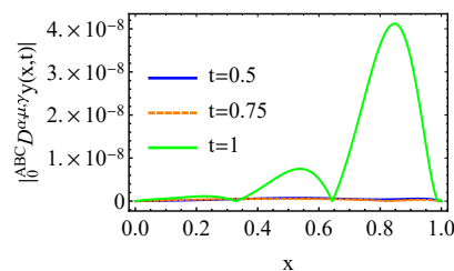
(b) The absolute ABC fractional derivative for Example 2 at \alpha = 1.9 .
