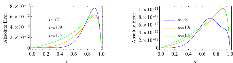
(a) The absolute error between the analytic solution and approximate solution for n = m = 10 with t = 0.5 .
