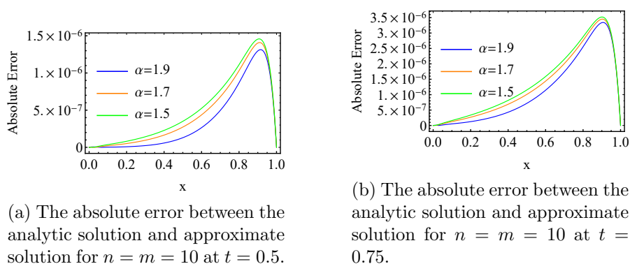
Figure 6: Graph the absolute error of Example 3 for n = m = 10 in 2D and in 3D with \alpha \rightarrow 2 and \mu = \gamma = 1 .
