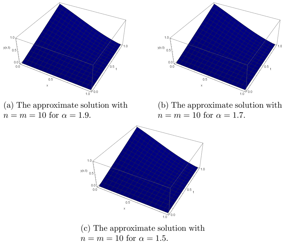
Figure 3: Graph of 3D approximate solutions y(x, t) of Example 2 for different fractional orders \alpha and \mu = \gamma = 1 .
