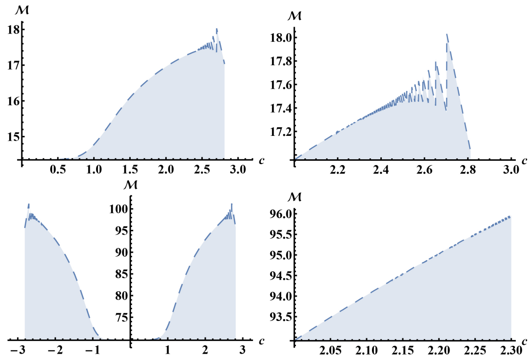
Figure 3: This figure illustrates the stability analysis of the solitary wave solutions (Eqs. (9), (14)) derived from both the Khat III and EKud methods. The plots display the momentum ((20), and (21)) as a function of various parameters, highlighting the conditions under which the wave solutions maintain stability.
