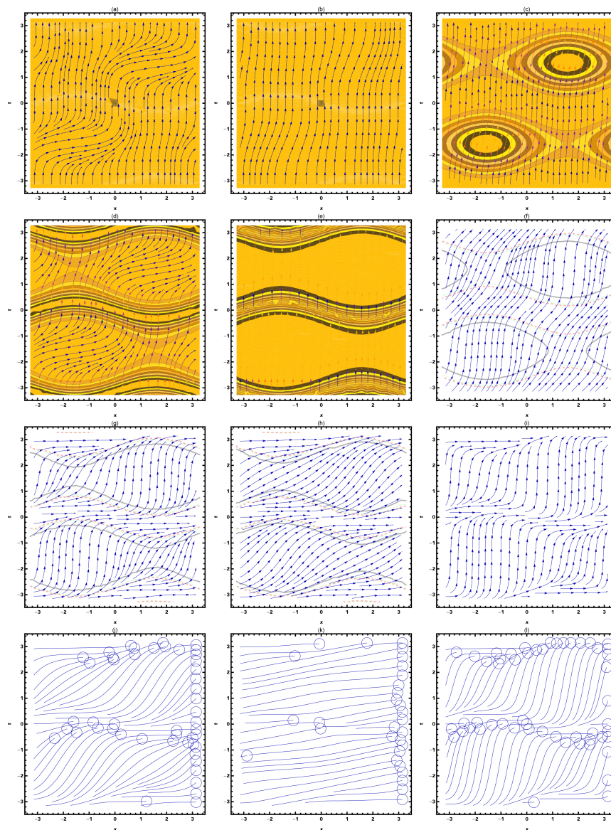
Figure 4: This stream plot illustrates the propagation of the solitary wave solution derived using the employed analytical methods. The arrows indicate the flow direction of the wave, while the color gradient represents the wave's intensity and amplitude, with warmer colors signifying higher amplitudes and cooler colors denoting lower amplitudes. The physical meaning of the plot reflects the interaction between short and long waves within the nonlinear system, capturing the wave's stable propagation over time and its energy distribution across the spatial domain
